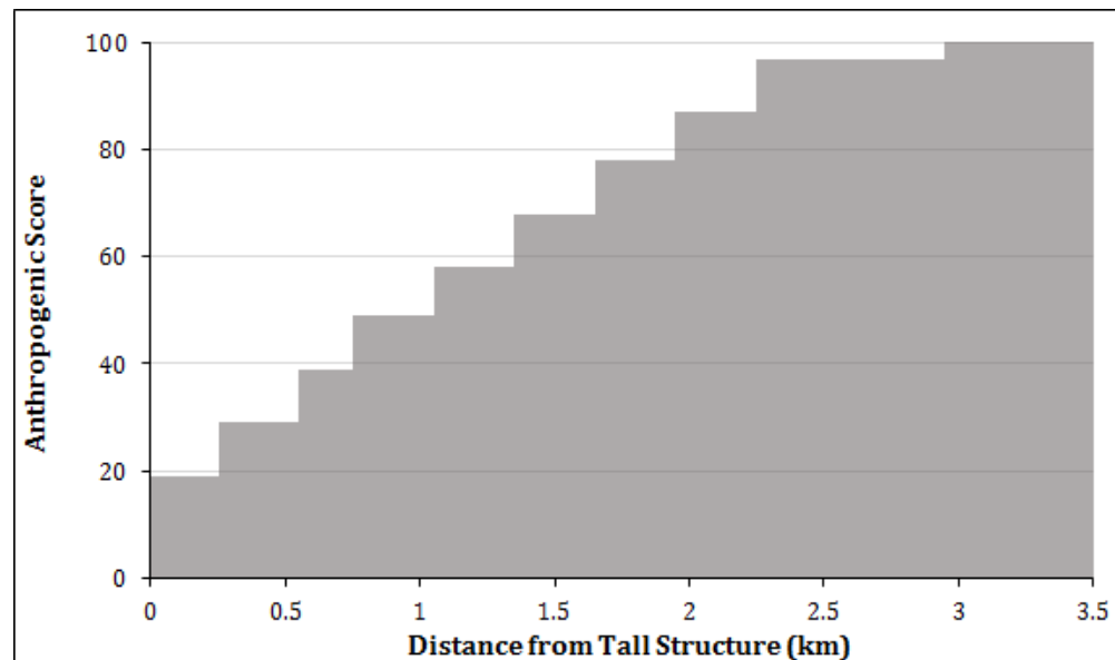
Figure C. 7. The Anthropogenic Score for Tall Structures located > 4-miles of an active sage-grouse lek that are considered non-nest facilitating structures for computing the Distance to Tall Structures Anthropogenic Variable.
