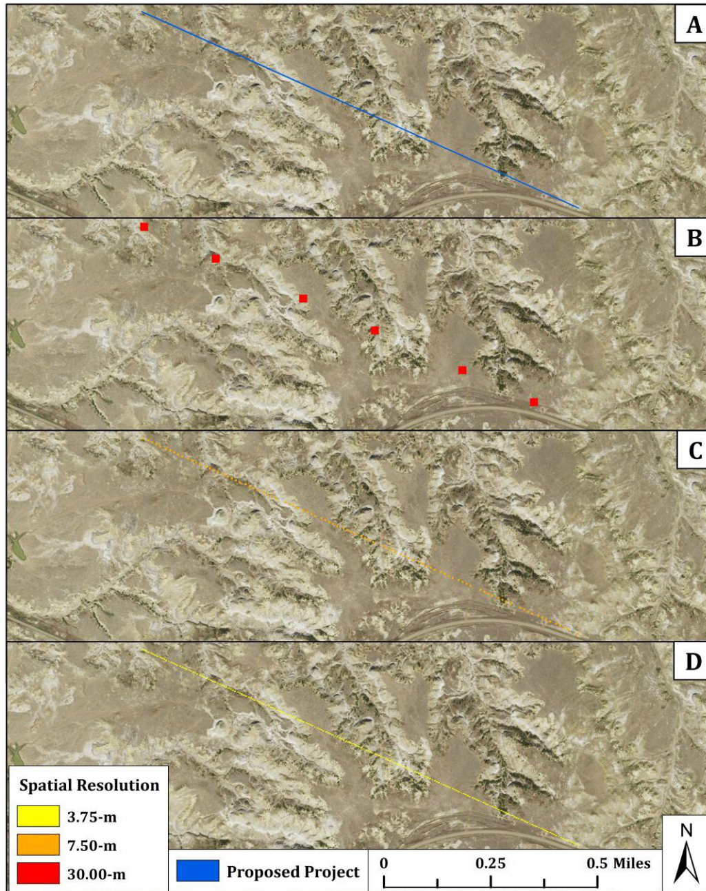
Figure 3. 1. Example of a proposed linear project showing the Direct Impact area (direct footprint; A) in blue covering approximately 1.30-acres. When converted to a raster data type with a 30.0 m (red; B) spatial resolution, the area for the HQT analysis increases to approximately 1.33-acres and covers areas outside of the project footprint, as well as excludes entire portions of the proposed project footprint. The amount of area missing decreases when converting to rasters with 7.50 m (orange; C) or 3.75 m (yellow; D) spatial resolutions, where the Direct Impact area for the HQT analysis very minimally increases by 0.003-acres for both resolutions.
