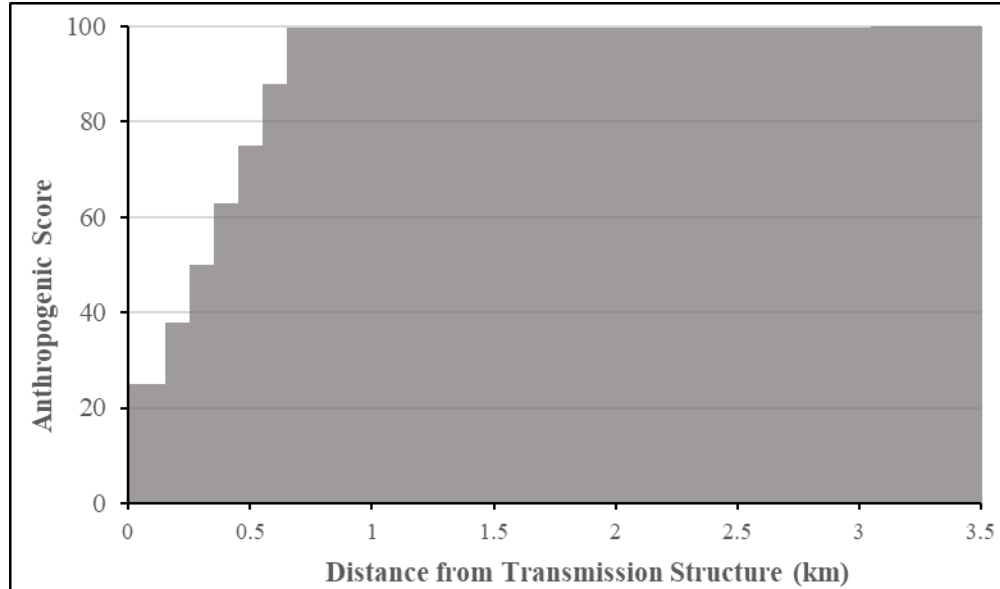
Figure D. 9. The Anthropogenic Score for Sub-Transmission/Distribution Structures \leq 69 kV that are considered non-nest facilitating structures for computing the Distance to Transmission/Distribution Structures Anthropogenic Variable.
