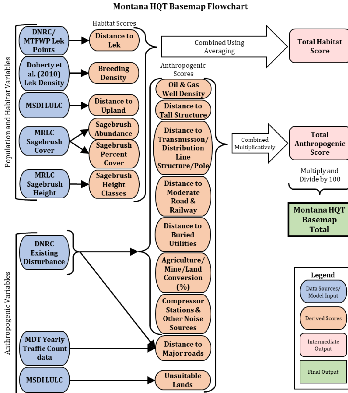
Figure A. 1. Flowchart showing the steps of data manipulations to develop the Montana HQT Basemap.
